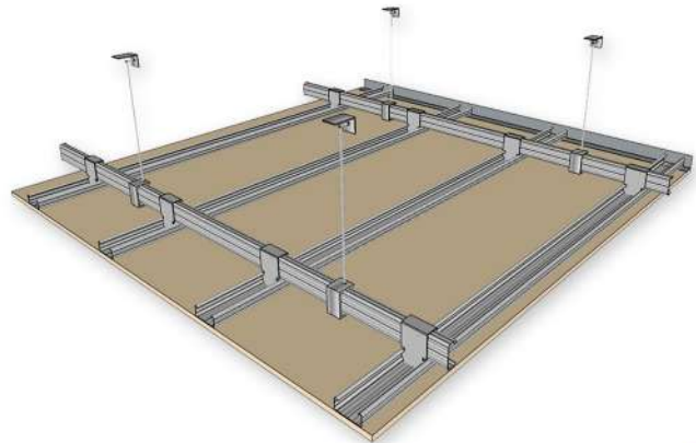
CONCEALED CEILING
