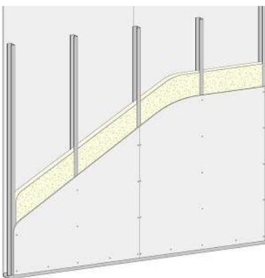
WALL PARTITION
